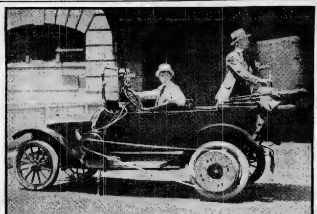
The above illustration shows the Maxwell automobile doing rather a unique performance. This particular Maxwell is equipped with a moving picture apparatus, which is run by the power of the Maxwell's engine. A pulley placed on the rear flywheel operates the electric equipment, and the variable speed gear saw machinery. This automobile was used in Atlanta last week, demonstrating to hundreds of people the efficiency of the Maxwell for such work. The car is touring the state of Georgia, doing the double work of entertaining those who see its performance and at the same time popularizing the Maxwell car.
